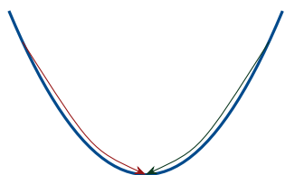
convex: any start, same floor
