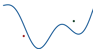
not convex: start picks the dip
